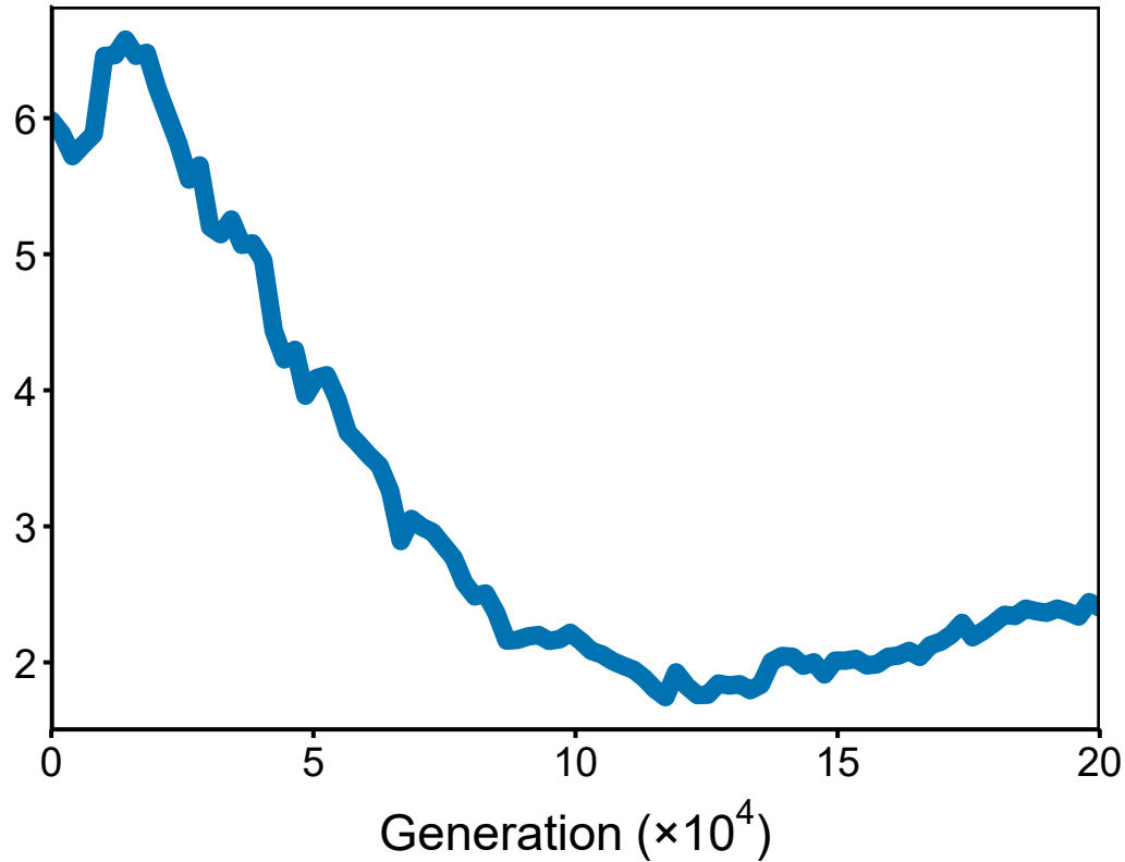
Mean absolute error from true coefficients
